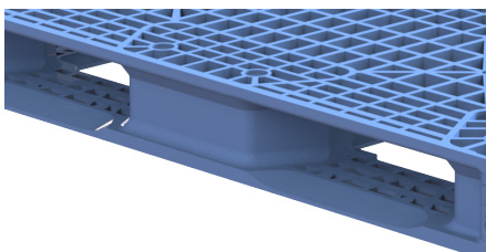
Narrower center block allows four-way entry
