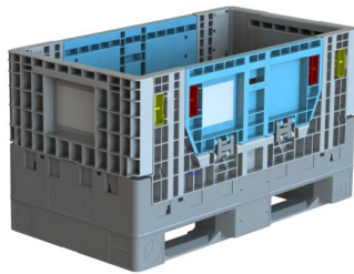
Two Drop Access Doors (Long Side)
